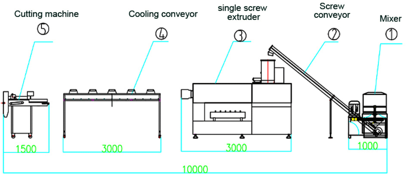
Layout of The Pet Treat Food Processing Line
